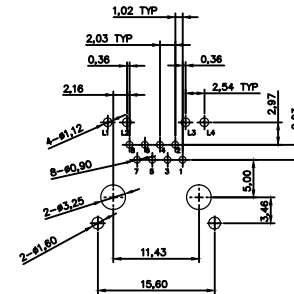
RECOMMENDED PCB LAYOUT (COMPONENT SIDE VIEW) TOLERANCE: ±0.05 [0.002]
